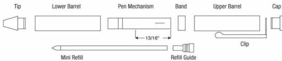
Diagram C - Assembly
